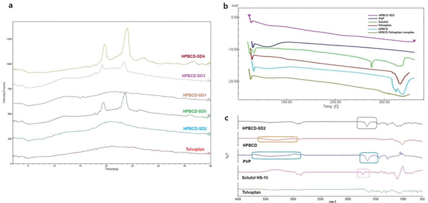
Figure 3. XRD diffractograms; (a) tolvaptan, HP \beta CD-SD1, HP \beta CD-SD2, HP \beta CD-SD3, HP \beta CD-SD4, HP \beta CD-SD5, and belonging to PVP, Solutol, tolvaptan, HP \beta CD, HP \beta CD-tolvaptan complex, and HP \beta CD-SD2; (b) DSC thermograms and (c) FTIR spectra.
